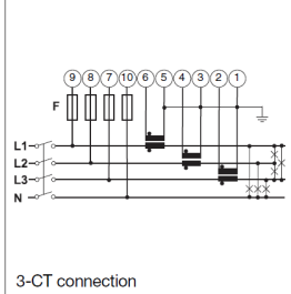
3-ph, 4-wire, unbalanced load Fig. 1
